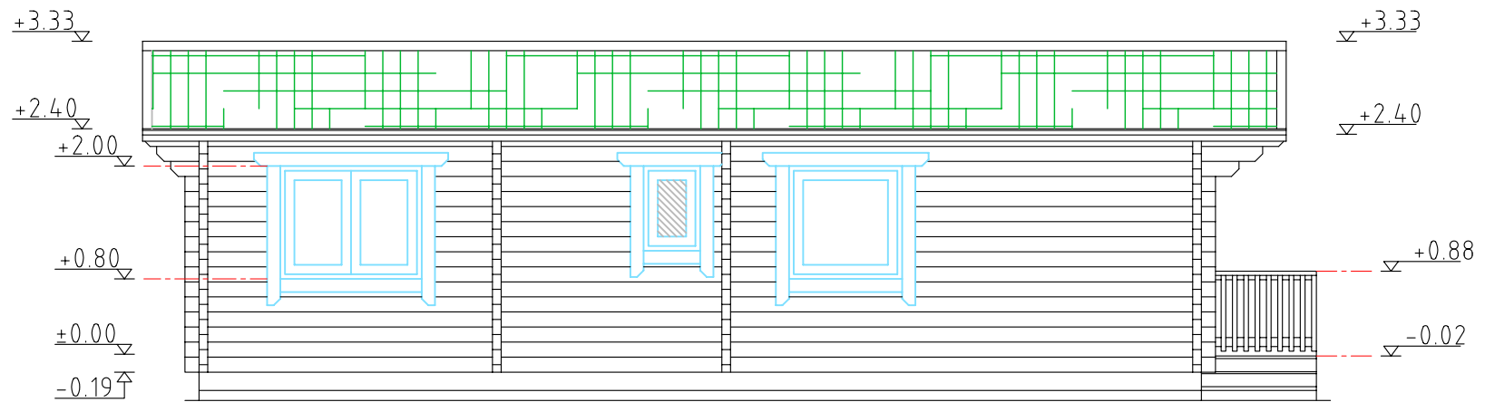
Elevation – B
