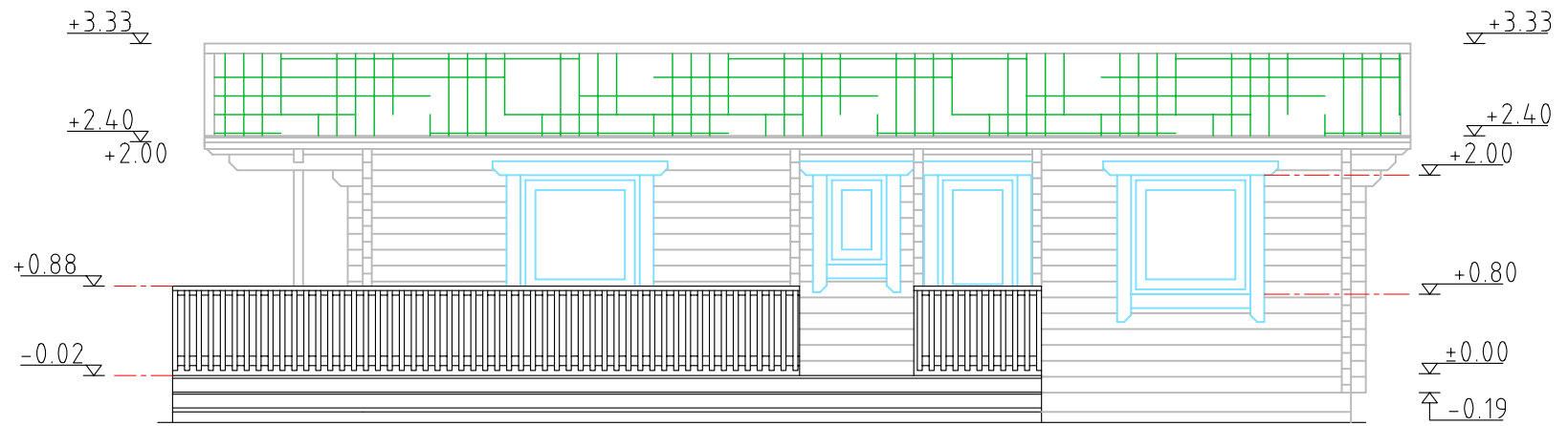
Elevation- A
